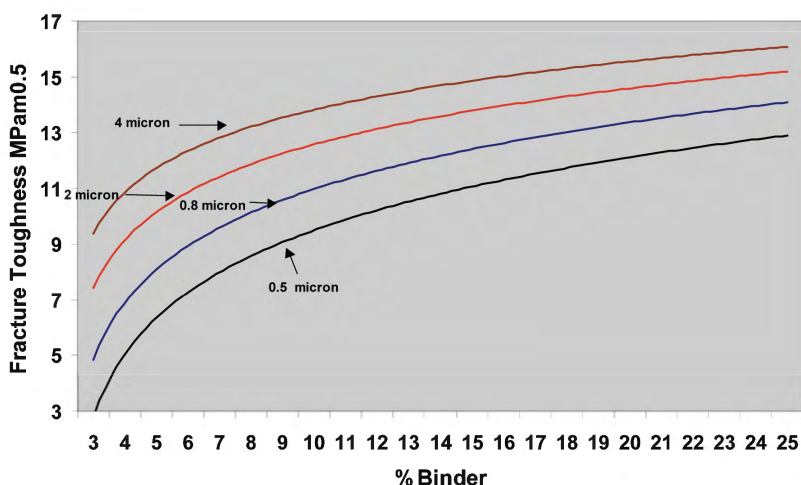
Fracture Toughness vs Grain Size
